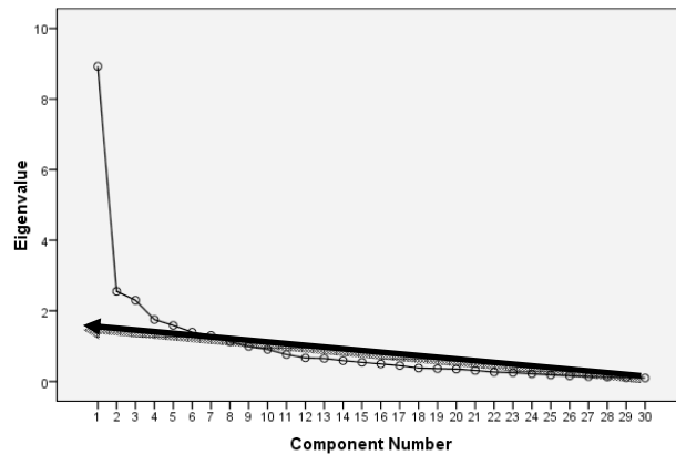
Scree Plot
