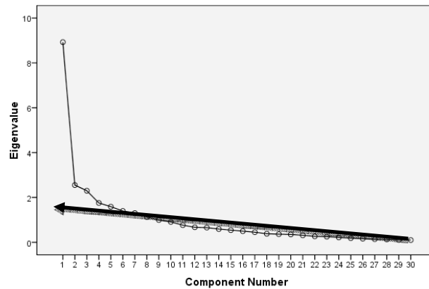
Scree Plot
